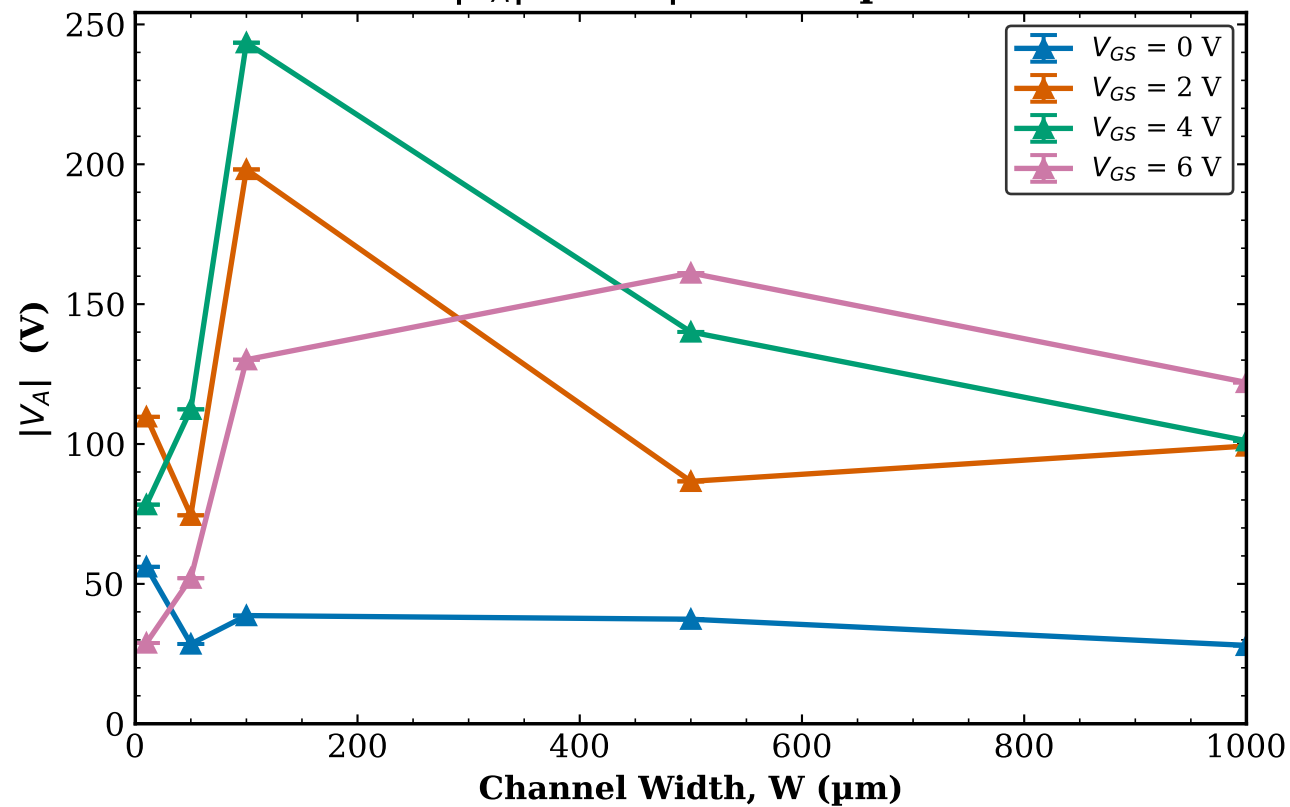
TFT1 Transistor 2 |V_A| vs W | L = 20\text{ }\mu\text{m}
